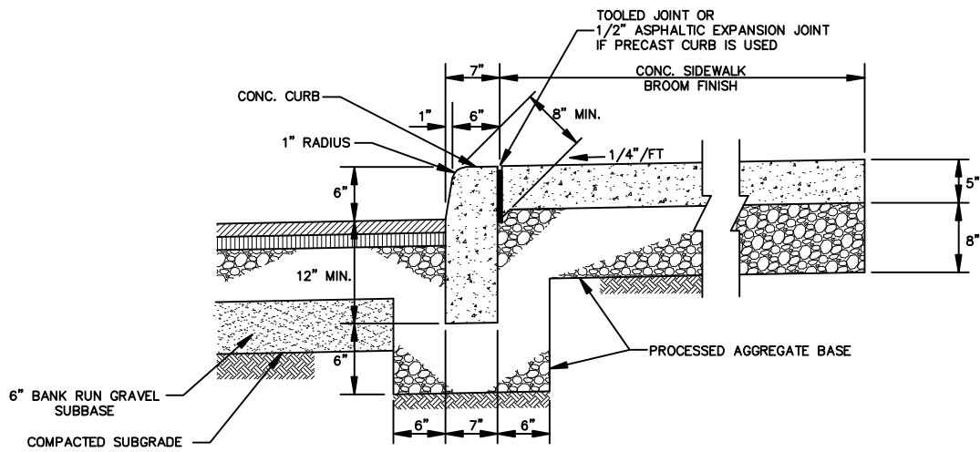
PAVEMENT/ SIDEWALK SECTION
