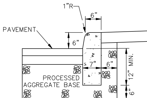
CONCRETE CURB
